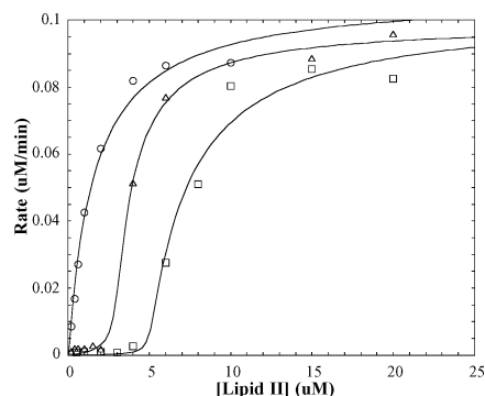
Figure 2. Rate of PBP1b versus the concentration of heptaprenyl Lipid II in the absence (○) and presence of ramoplanin (△ = 6 \mu\text{M} 1 ; □ = 8 \mu\text{M} 1 ).
